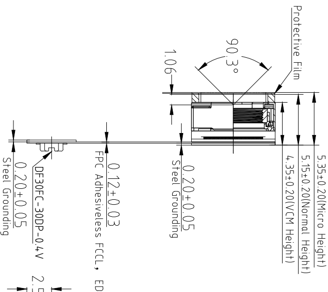
SIDE VIEW
